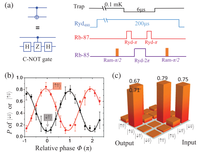
FIG. 4. Heteronuclear CNOT gate. (a) Experimental time sequence. (b) Output states as a function of the relative phase between the Raman \pi/2 pulses, for the initial states |\downarrow\downarrow\rangle (black squares) and |\uparrow\uparrow\rangle (red circles). The solid curves are sinusoidal fits yielding the phase difference of (0.94 \pm 0.01)\pi between the two signals. (c) Measured truth table matrix U_{\text{CNOT}} for the CNOT gate with the relative phase between the \pi/2 pulses set to 0.
